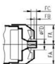
入力軸帶風扇 Input Shaft With fan
