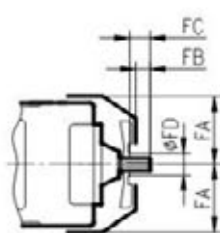
入力軸帶風扇 Input Shaft With fan
