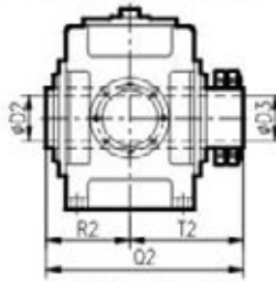
空心出力軸帶鎖盤型 Hollow Output Shaft (Shrink Disk Type)
