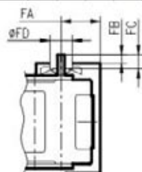
入力軸帶風扇 Input Shaft With fan
