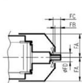
入力軸帶風扇 Input Shaft With fan
