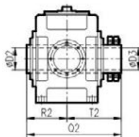
空心出力軸帶緊盤型 Hollow Output Shaft (Shrink Disk Type)
